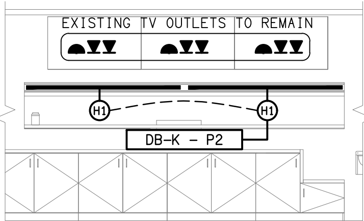
DETAIL B CAFE SERVERY ELEVATION SCALE 1:50
